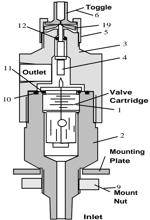
Model 1091 Toggle Valve
